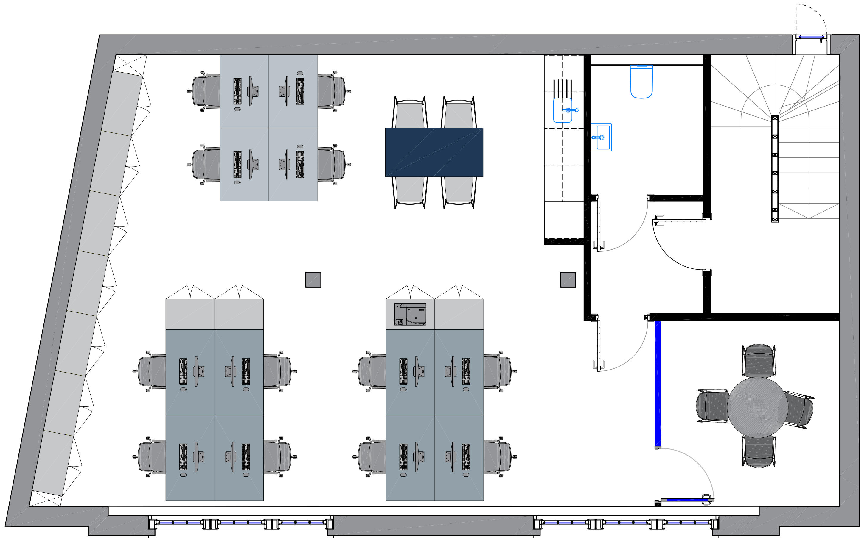
PROPOSED LAYOUT - UNIT 16 - FOUNDRY MEWS
